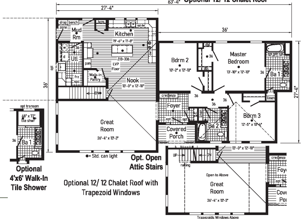
Proposed 2nd Floor with Optional 12/12 Chalet Roof
